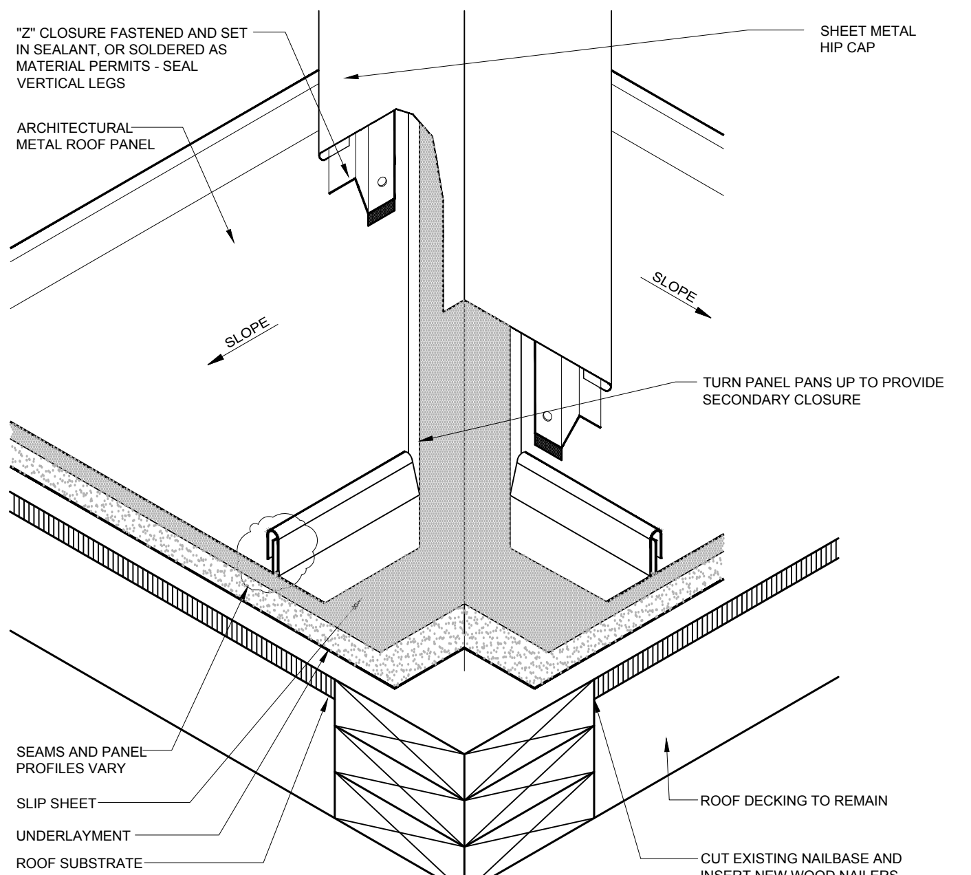
4 HIP & RIDGE EDGE FLASHING NOT TO SCALE
