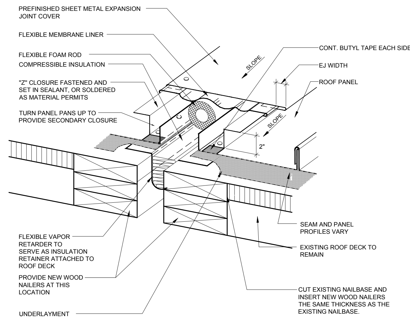
7 ROOF TO ROOF EXPANSION JOINT NOT TO SCALE
