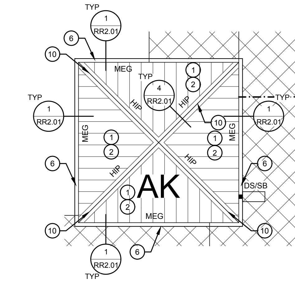
ENLARGED ROOF PLAN - ALT BID #2 RYAN HIGH SCHOOL
