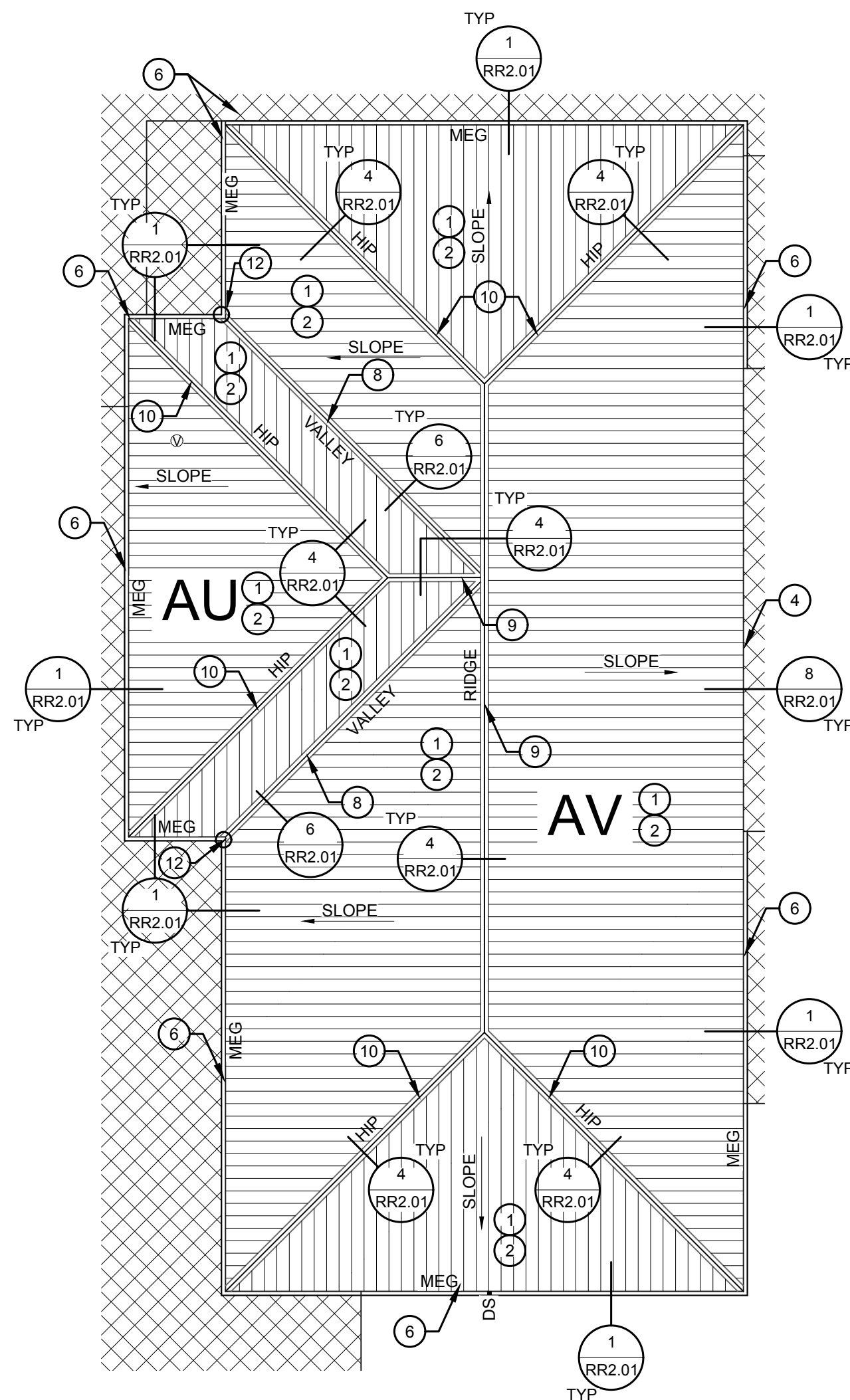
ENLARGED ROOF PLAN - ALT BID #3 RYAN HIGH SCHOOL
