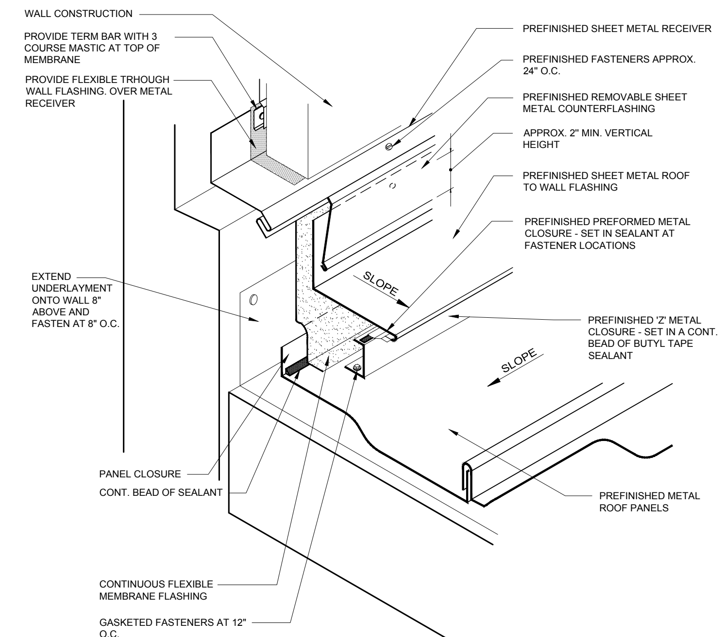
9 ROOF TO SIDE RISEWALL FLASHING NOT TO SCALE
