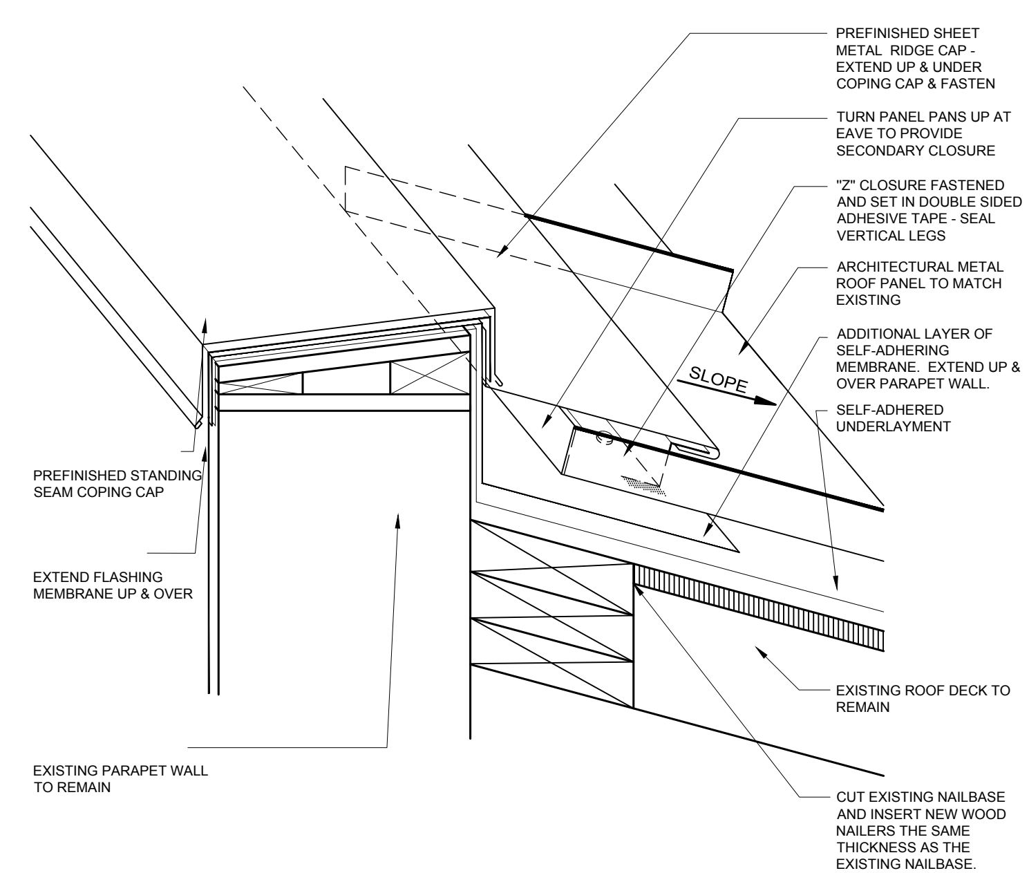
5 PARAPET AT HIGH EAVE NOT TO SCALE
