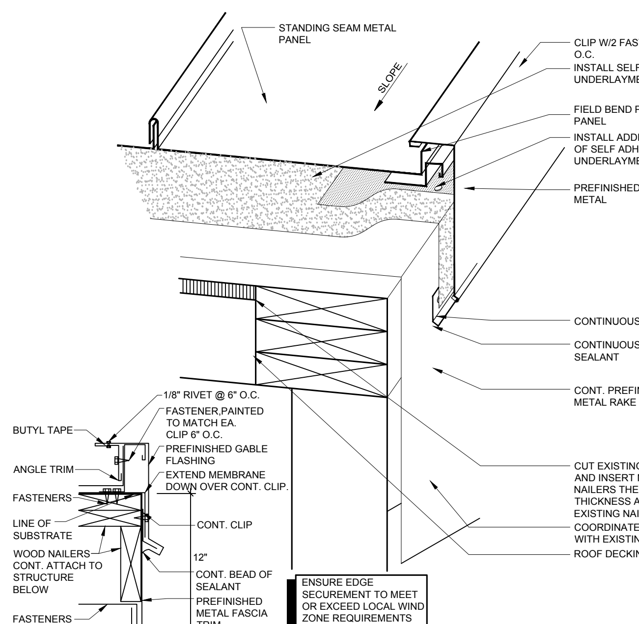
2 METAL EDGE RAKE NOT TO SCALE
