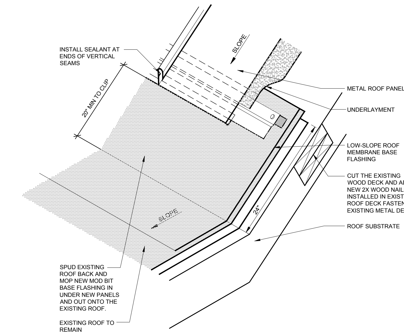
8 STANDING SEAM TO LOW SLOPE ROOF SYSTEM NOT TO SCALE
