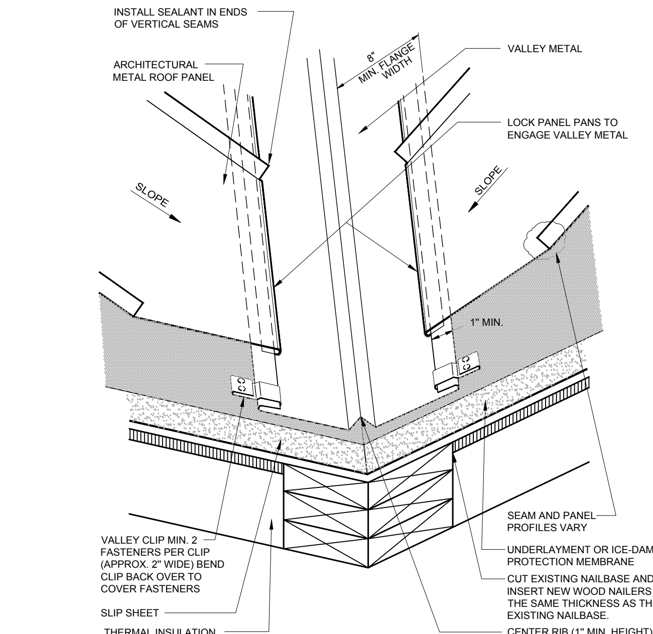
6 VALLEY NOT TO SCALE
