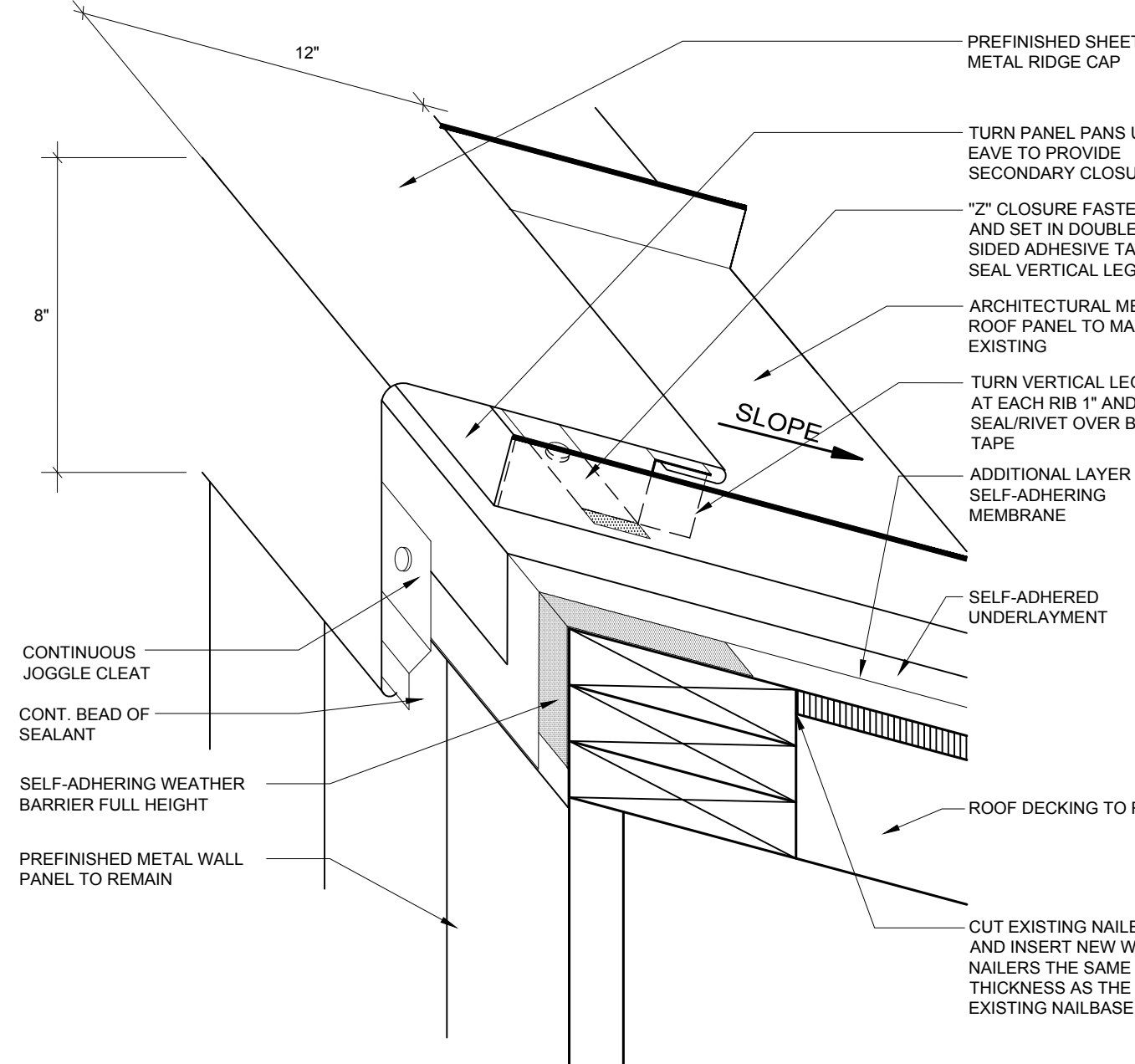
3 HIGH EAVE NOT TO SCALE
