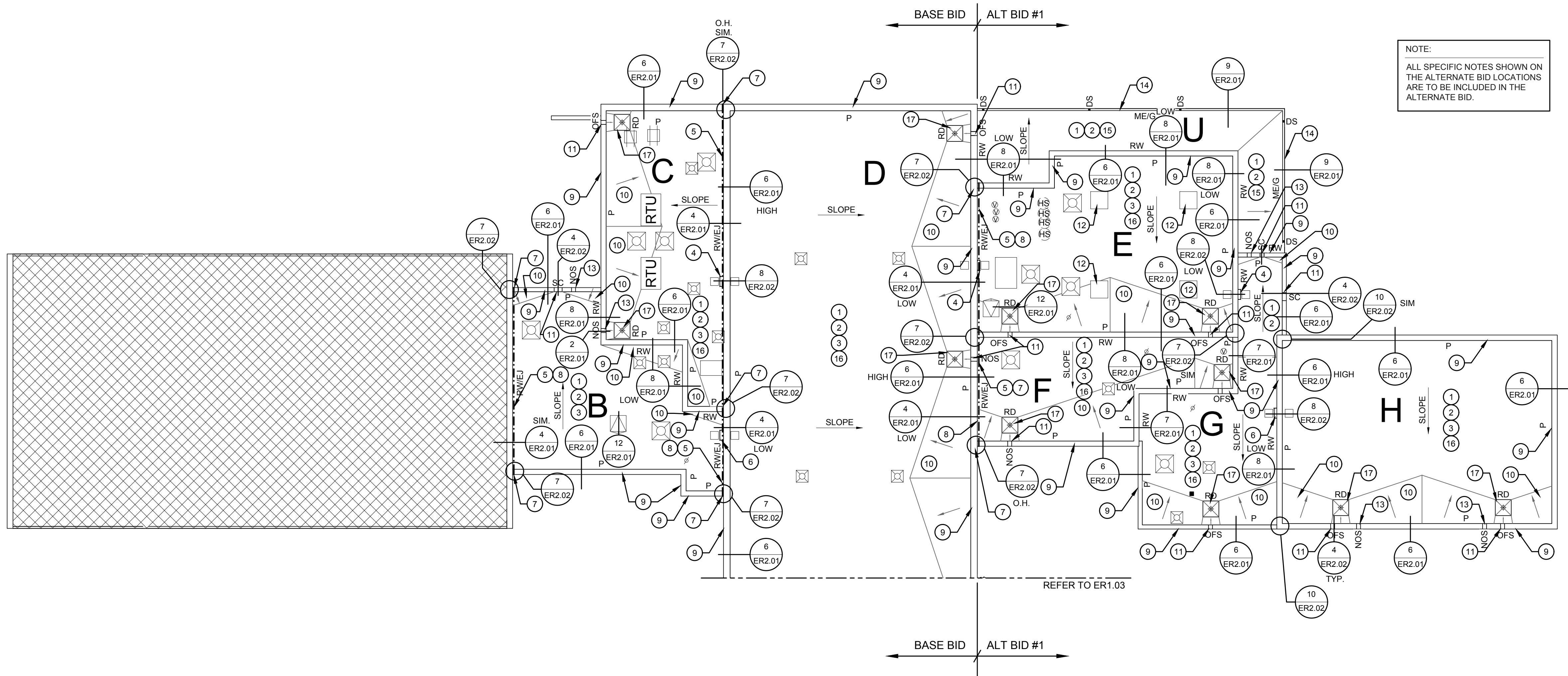
ENLARGED ROOF PLAN - BASE BID EVERS PARK ELEMENTARY SCHOOL 1 NOT TO SCALE
