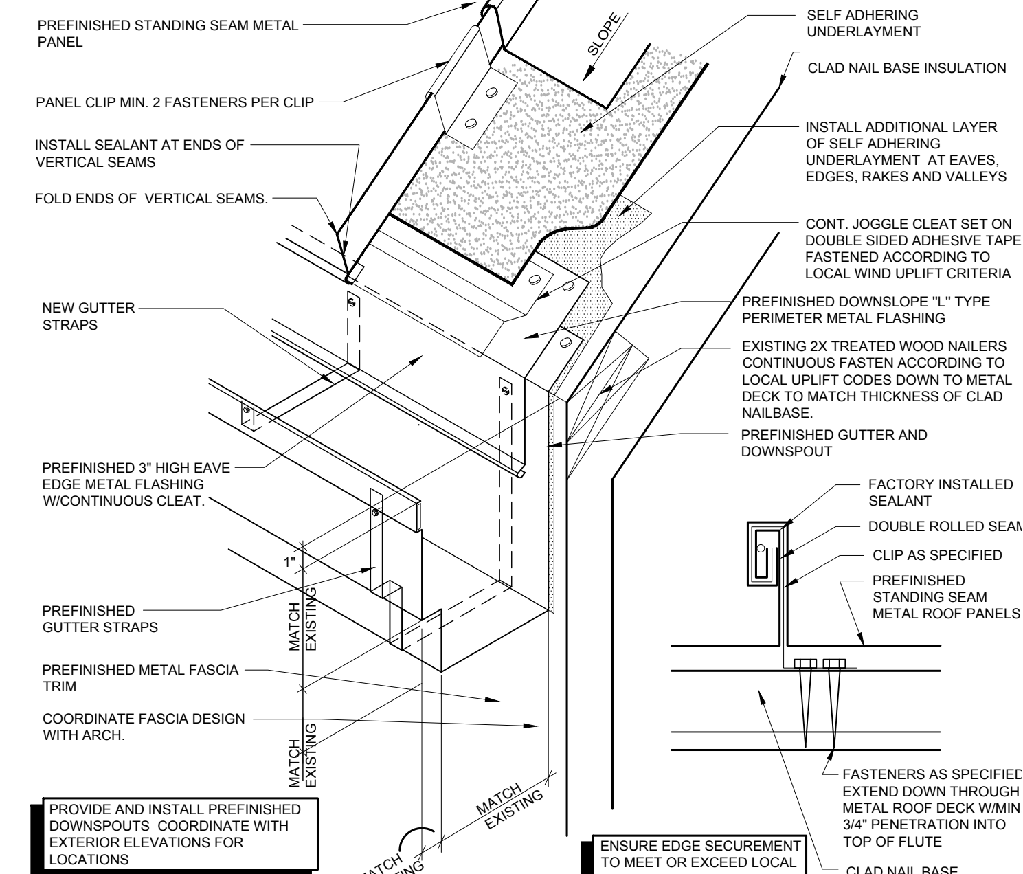
1 METAL EDGE WITH GUTTER PROFILE TO MATCH EXISTING NOT TO SCALE
